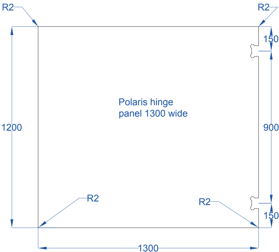
Polaris Glass to Glass Hinge Cut Out as per detail
