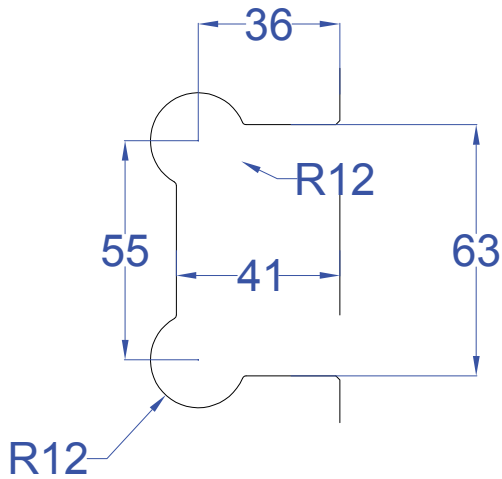
Polaris Glass to Glass Hinge Cut Out as per detail
